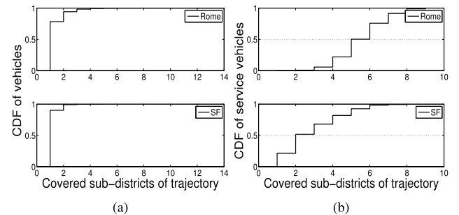
Fig. 3. Inter-district property of trajectories. (a) General vehicles. (b) Service vehicles.
