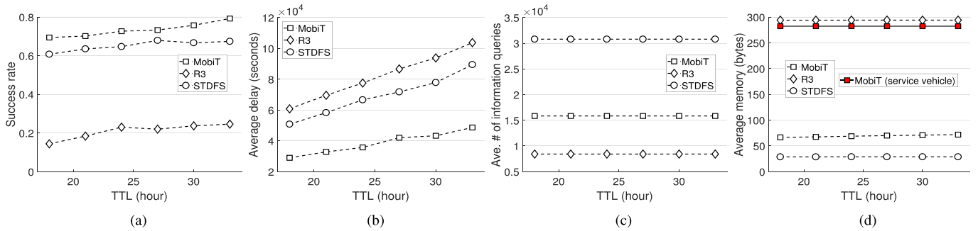
Fig. 12. Performance with different TTLs using the Rome trace. (a) Success rate. (b) Average delay. (c) Average number of info. queries. (d) Average memory usage.
