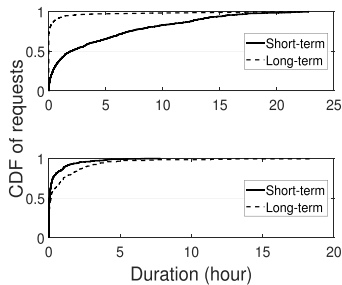
Fig. 16. Durations of using short-term and long-term mobility information.
