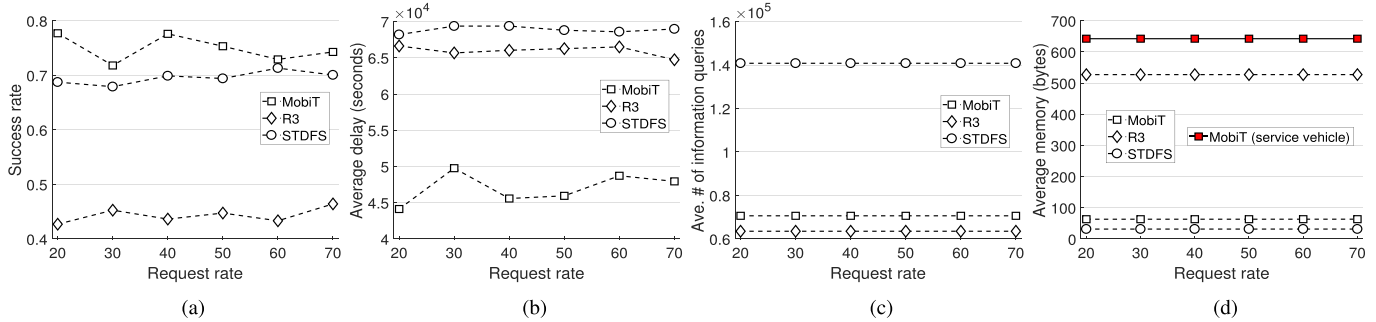
Fig. 11. Performance with different request rates using the San Francisco trace. (a) Success rate. (b) Average delay. (c) Average number of info. queries. (d) Average memory usage.
