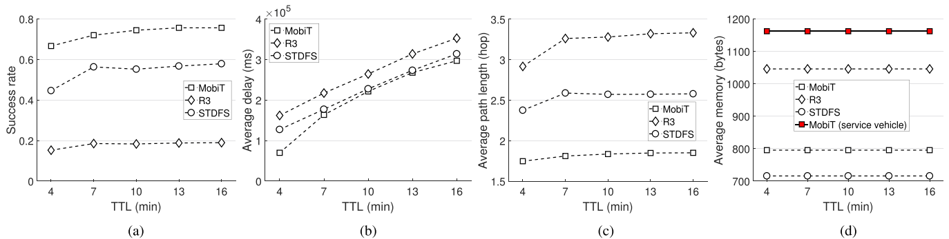
Fig. 18. Performance with different TTLs in real implementation. (a) Success rate. (b) Average delay. (c) Average path length. (d) Memory usage of vehicle.
