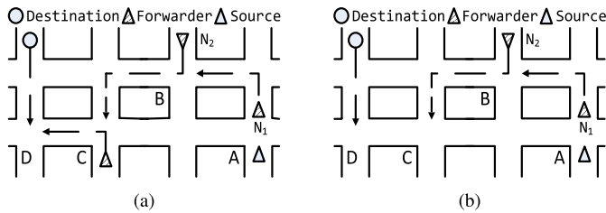
Fig. 9. Selection of forwarders. (a) Complete list of forwarders. (b) Incomplete list of forwarders.
