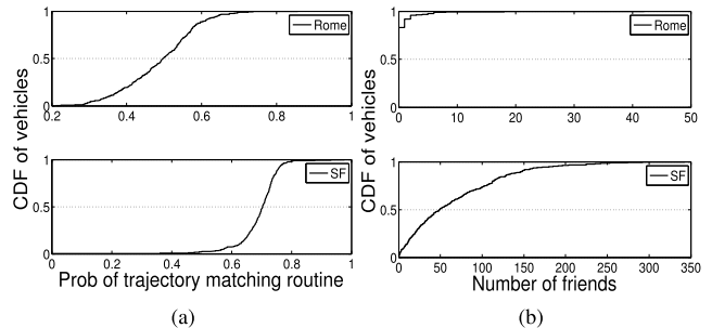
Fig. 2. Long-term mobility of vehicles. (a) Trajectory matches routine. (b) Number of friends.
