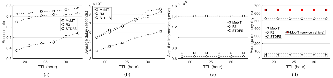
Fig. 13. Performance with different TTLs using the San Francisco trace. (a) Success rate. (b) Average delay. (c) Average number of info. queries. (d) Average memory usage.
